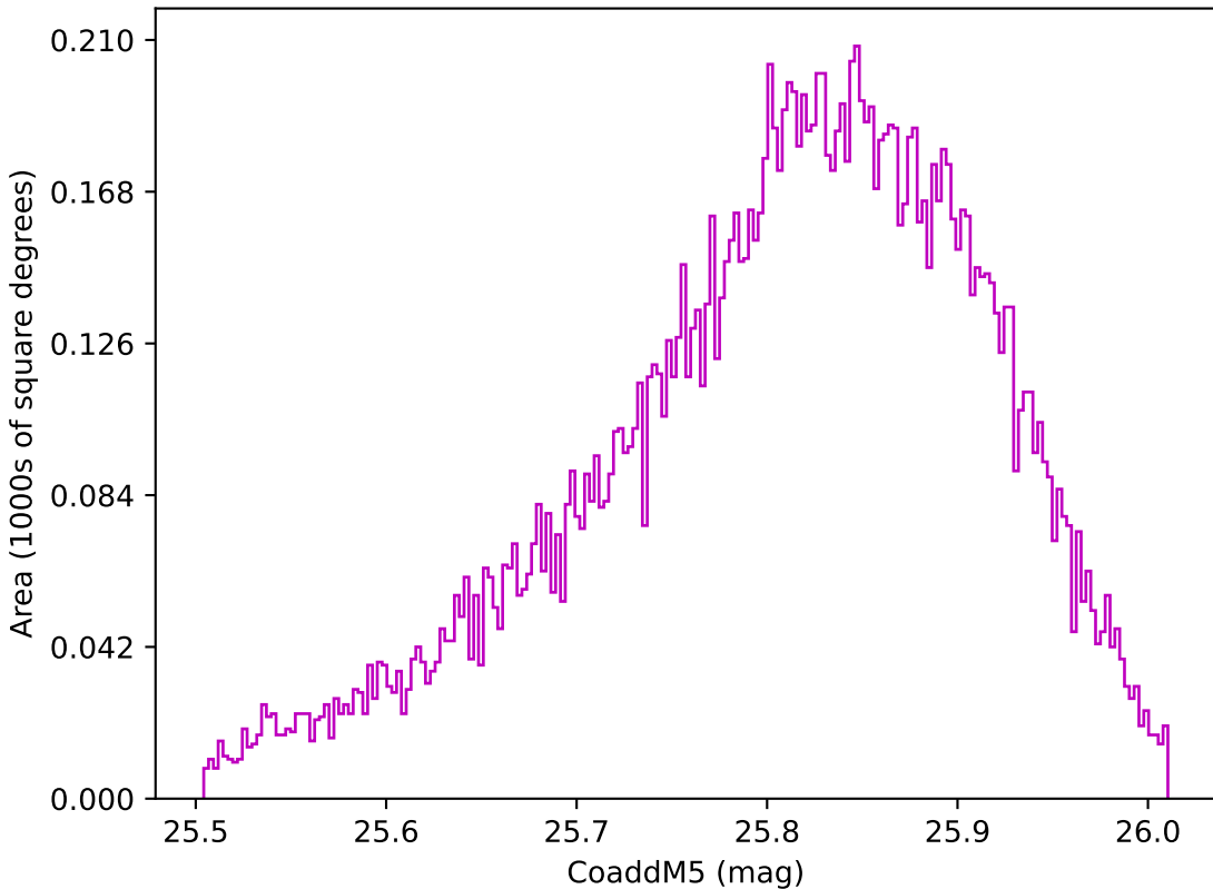
too_elab_r8_d2_ugrizy_v3.4_10yrs WFD z band: CoaddM5
