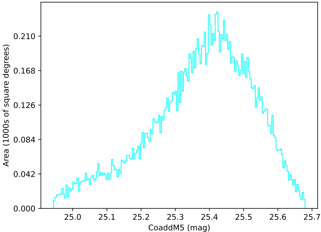
too_elab_r8_d2_ugrizy_v3.4_10yrs WFD u band: CoaddM5
