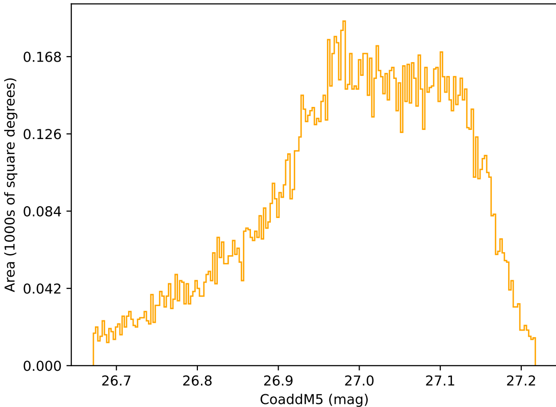
too_elab_r8_d2_ugrizy_v3.4_10yrs WFD r band: CoaddM5
