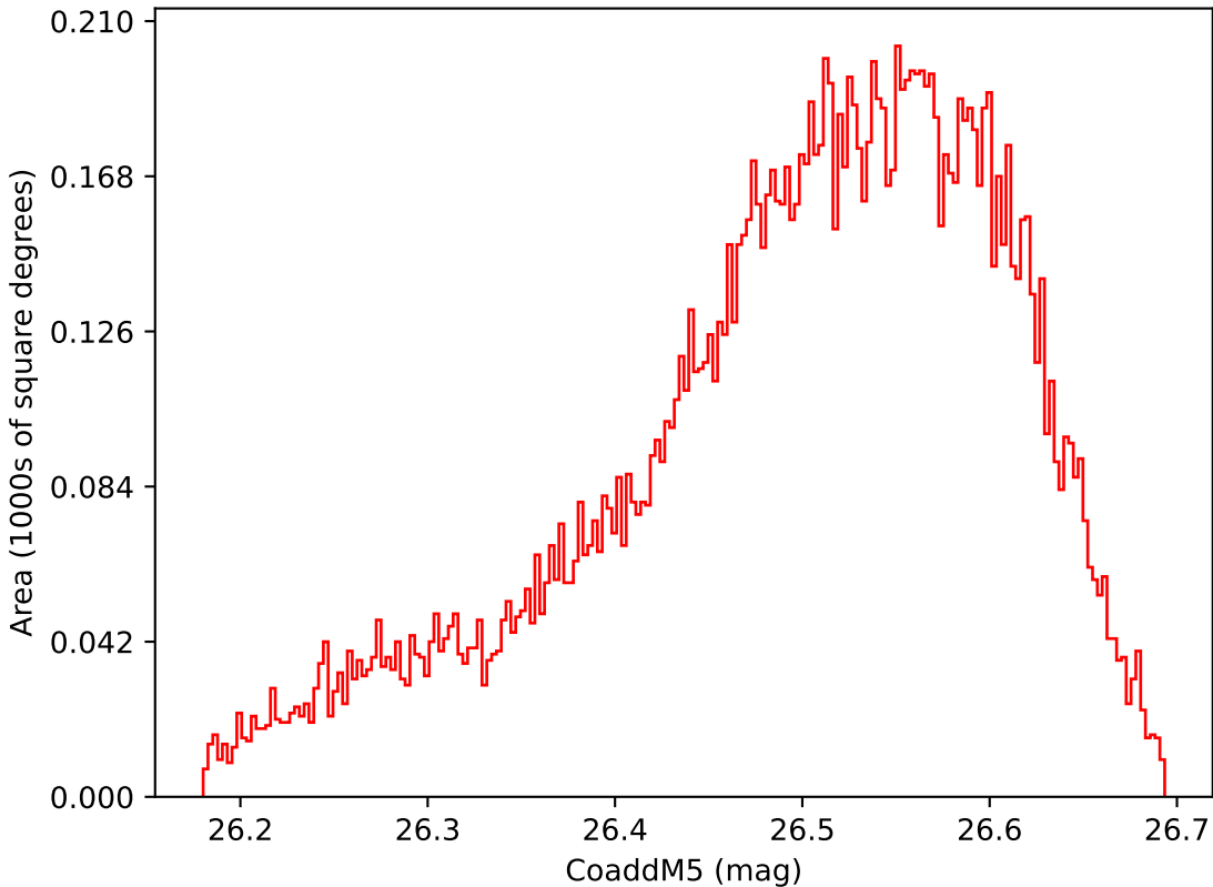
too_elab_r8_d2_ugrizy_v3.4_10yrs WFD i band: CoaddM5
