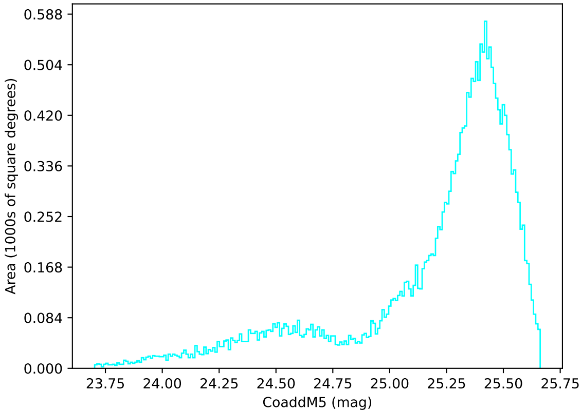
too_elab_r8_d2_ugrizy_v3.4_10yrs All sky u band: CoaddM5
