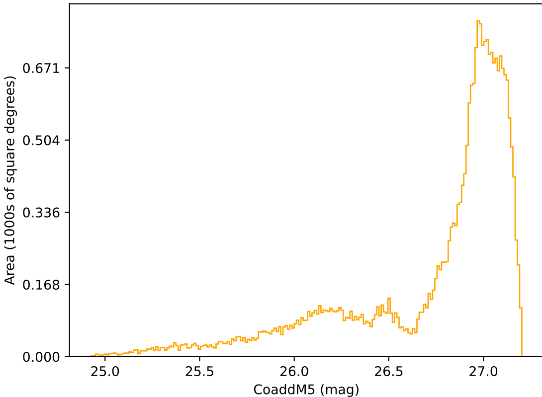
too_elab_r8_d2_ugrizy_v3.4_10yrs All sky r band: CoaddM5
