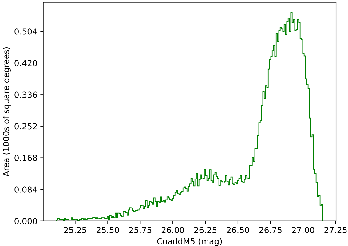
too_elab_r8_d2_ugrizy_v3.4_10yrs All sky g band: CoaddM5
