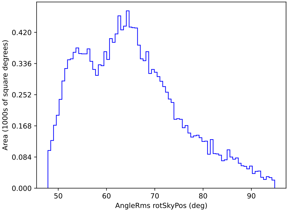
too_elab_r8_d2_ugrizy_v3.4_10yrs WFD z band: AngleRms rotSkyPos
