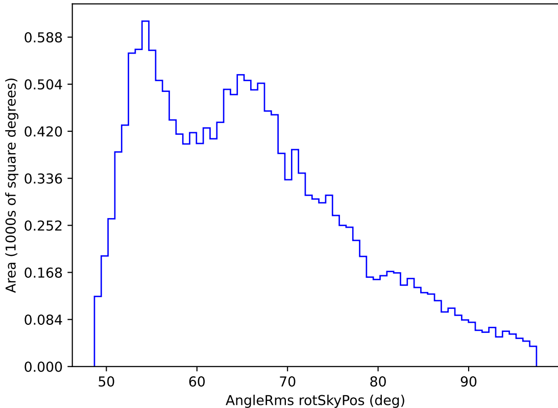
too_elab_r8_d2_ugrizy_v3.4_10yrs WFD r band: AngleRms rotSkyPos
