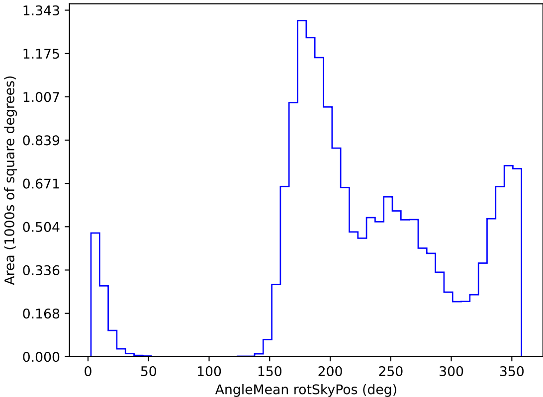
too_elab_r8_d2_ugrizy_v3.4_10yrs WFD u band: AngleMean rotSkyPos
