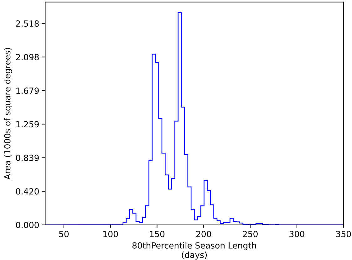
too_elab_r8_d2_ugrizy_v3.4_10yrs WFD y band: 80thPercentile Season Length
