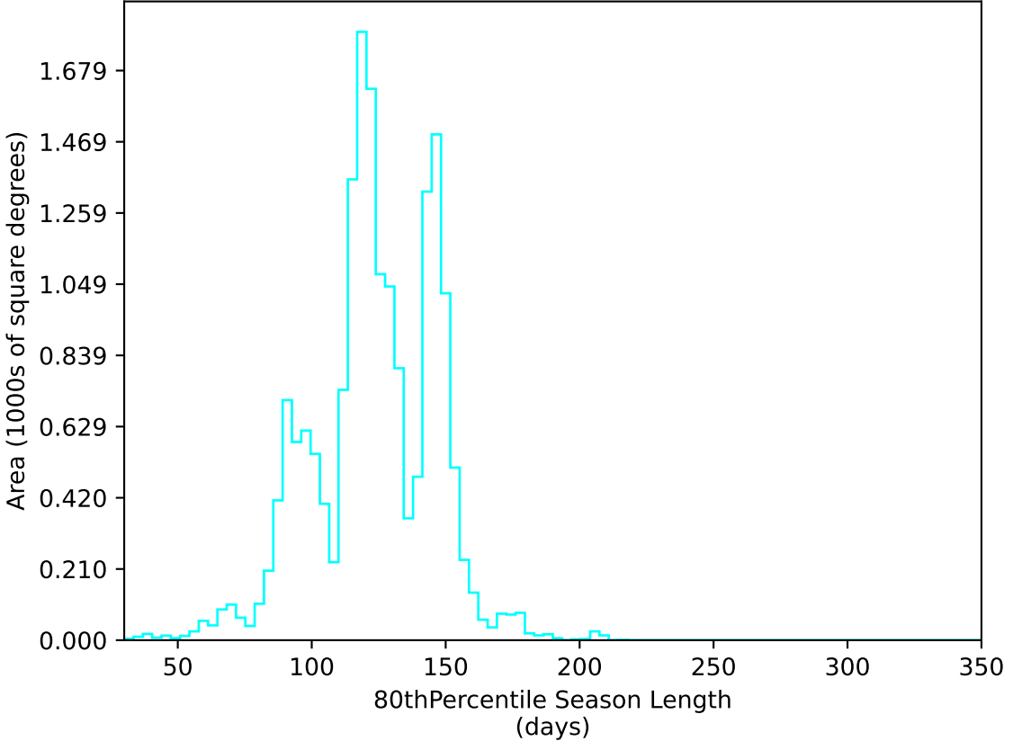
too_elab_r8_d2_ugrizyv3.4_10yrs WFD u band: 80thPercentile Season Length
