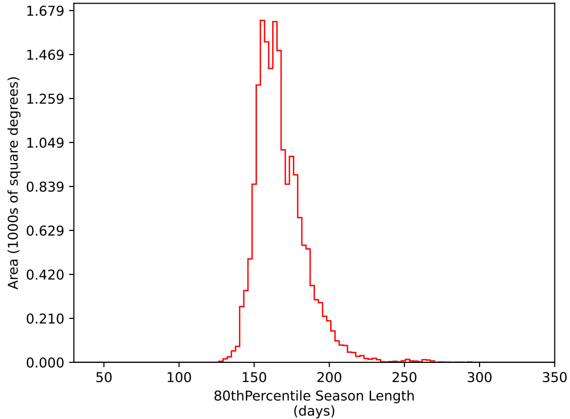
too_elab_r8_d2_ugrizy_v3.4_10yrs WFD i band: 80thPercentile Season Length
