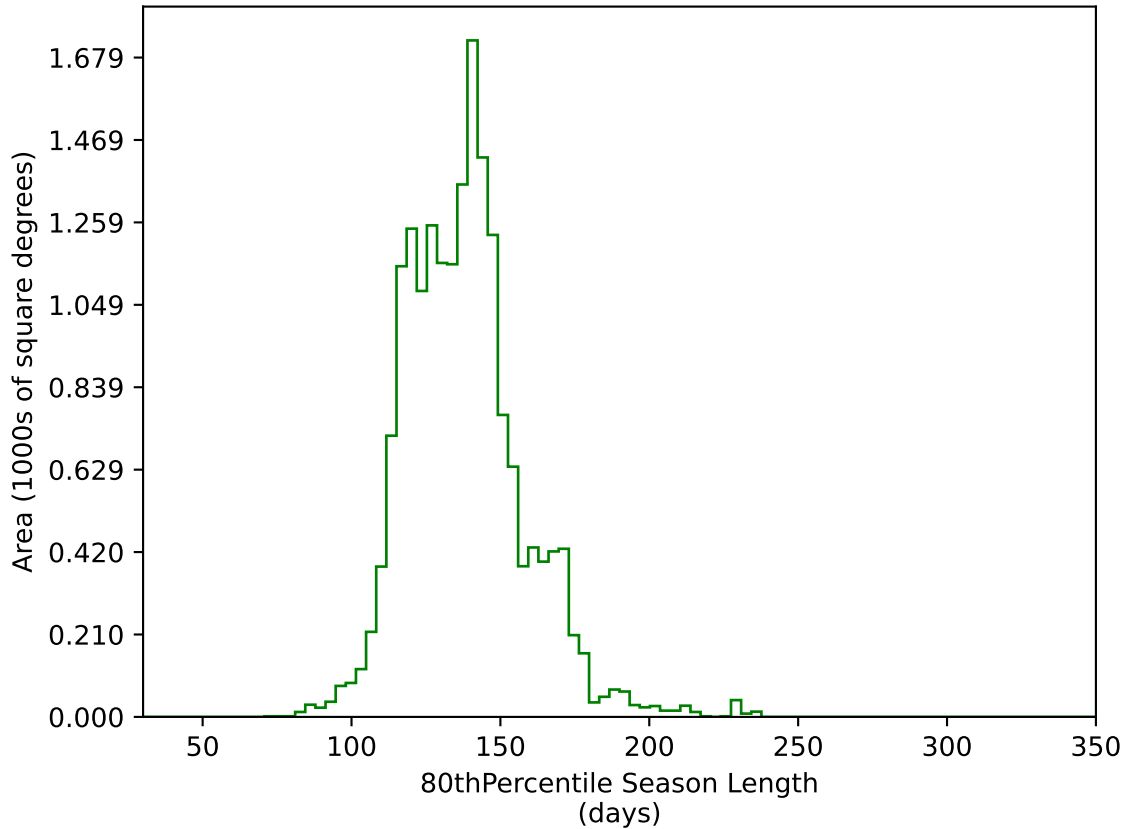
too_elab_r8_d2_ugrizy_v3.4_10yrs WFD g band: 80thPercentile Season Length
