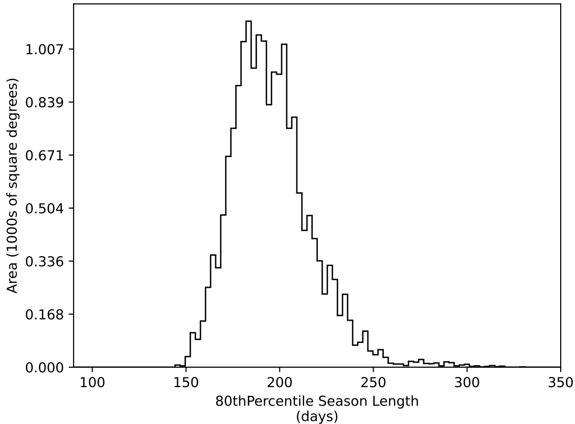
too_elab_r8_d2_ugrizy_v3.4_10yrs WFD all bands: 80thPercentile Season Length
