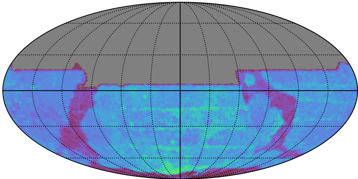
too_elab_r8_d2_ugrizy_v3.4_10yrs All sky y band: 80thPercentile Season Length
