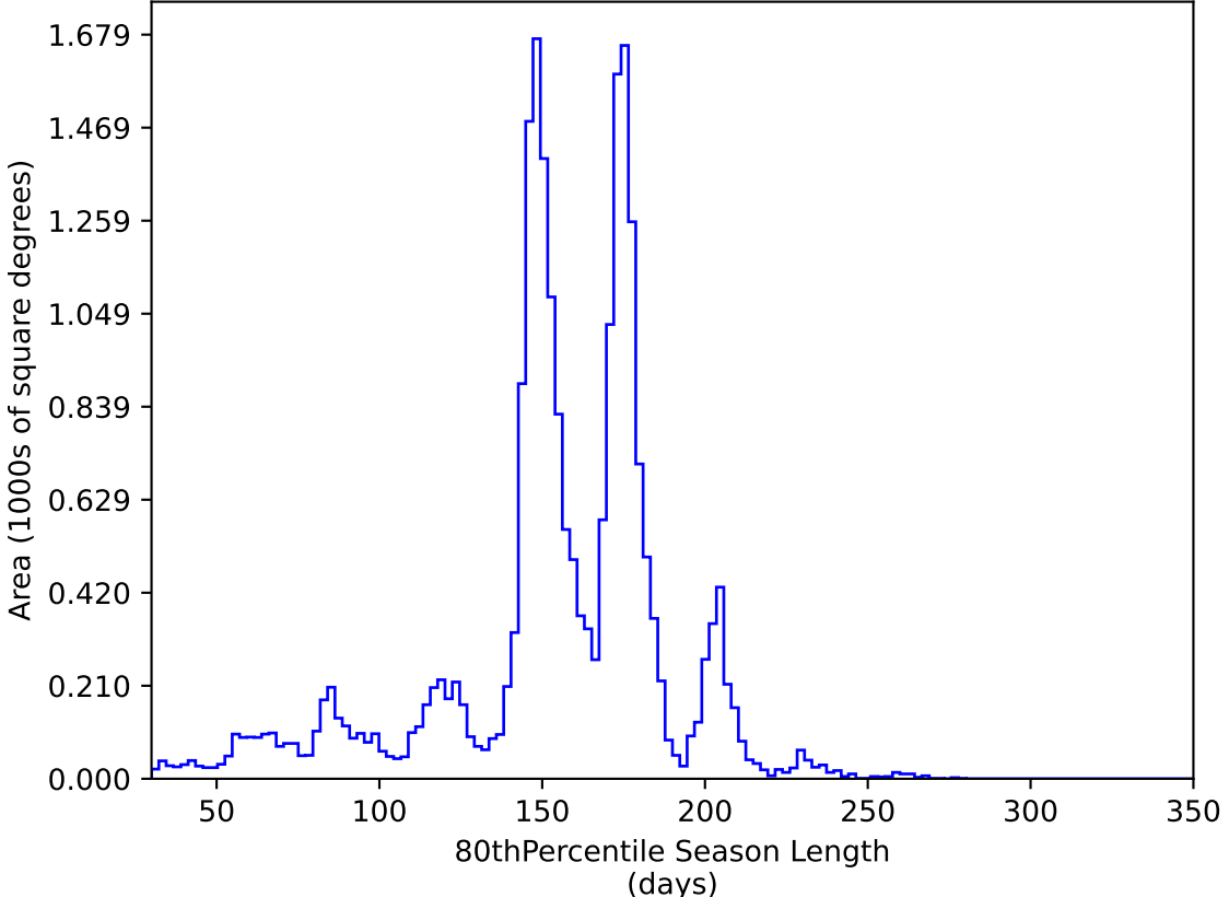
too_elab_r8_d2_ugrizy_v3.4_10yrs All sky y band: 80thPercentile Season Length
