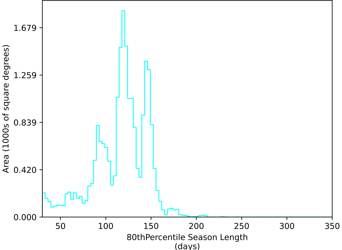
too_elab_r8_d2_ugrizy_v3.4_10yrs All sky u band: 80thPercentile Season Length
