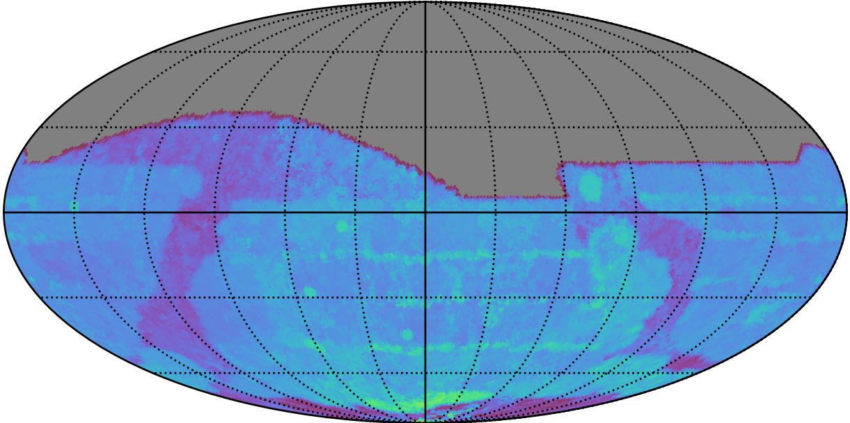
too_elab_r8_d2_ugrizy_v3.4_10yrs All sky i band: 80thPercentile Season Length
