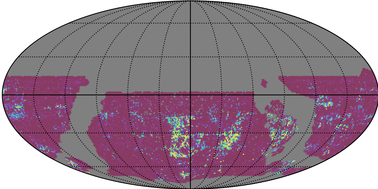
too_elab_r8_d2_ugrizy_v3.4_10yrs WFD u band: 75th Percentile Intranight Timespan
