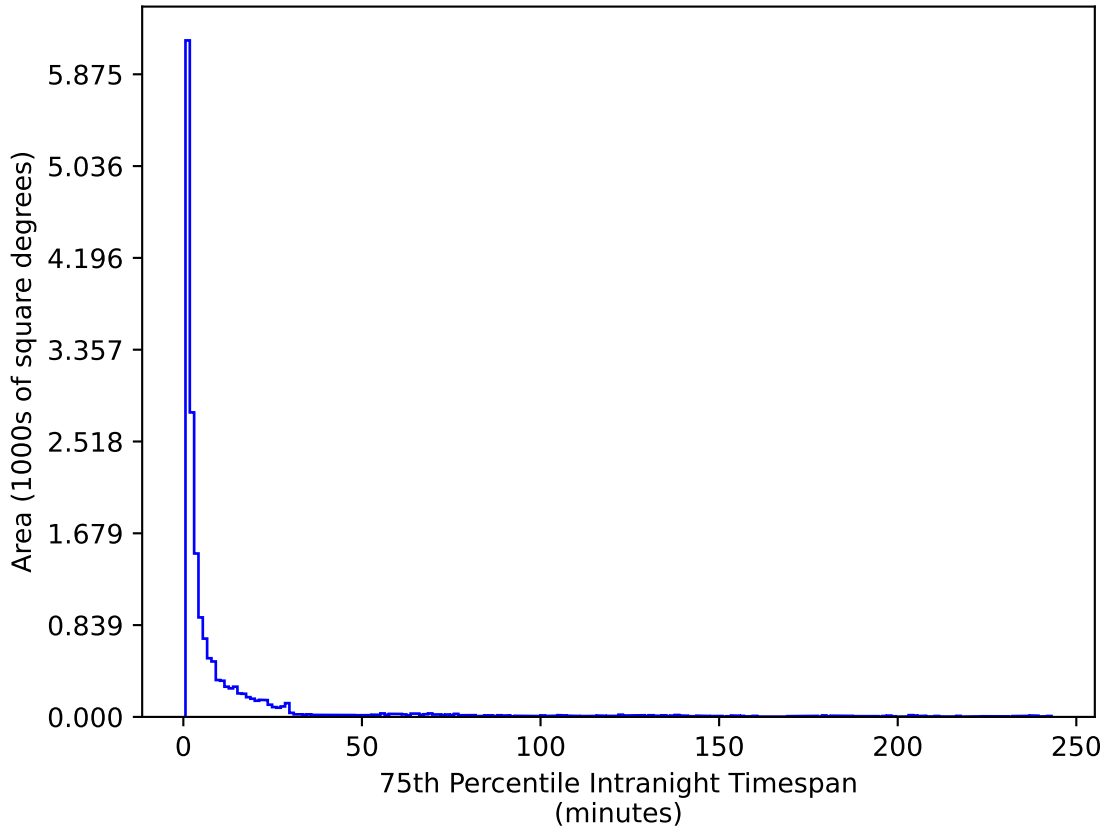
too_elab_r8_d2_ugrizy_v3.4_10yrs WFD u band: 75th Percentile Intranight Timespan
