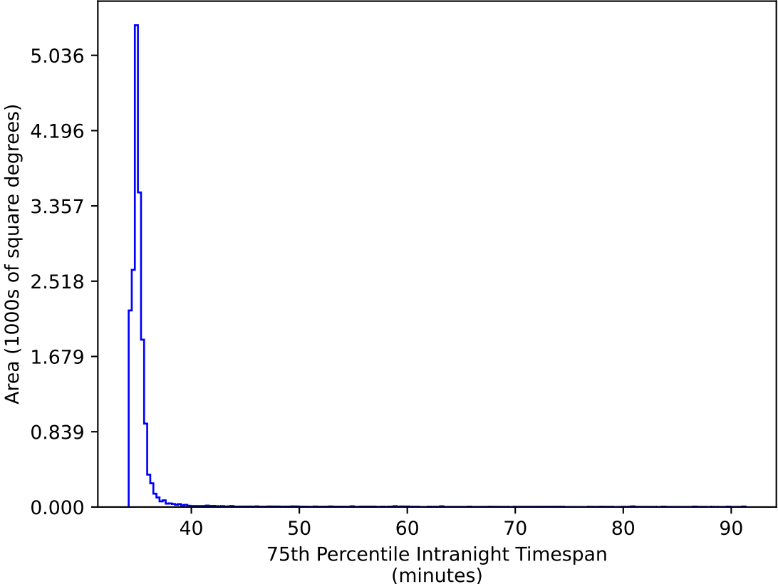
too_elab_r8_d2_ugrizy_v3.4_10yrs WFD ri bands: 75th Percentile Intranight Timespan
