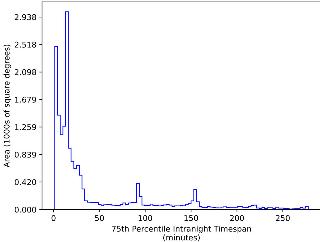
too_elab_r8_d2_ugrizy_v3.4_10yrs WFD r band: 75th Percentile Intranight Timespan
