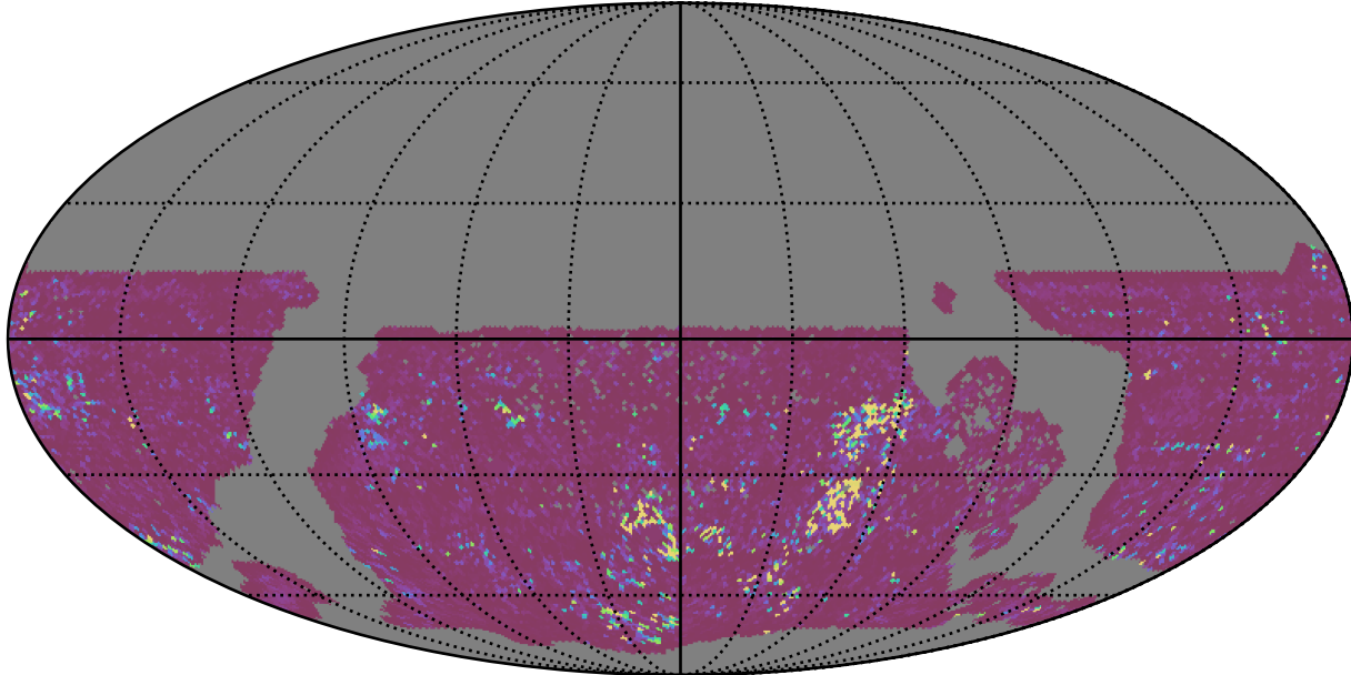
too_elab_r8_d2_ugrizy_v3.4_10yrs WFD g band: 75th Percentile Intranight Timespan
