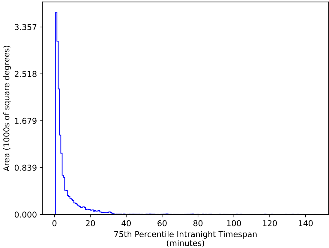
too_elab_r8_d2_ugrizy_v3.4_10yrs WFD g band: 75th Percentile Intranight Timespan
