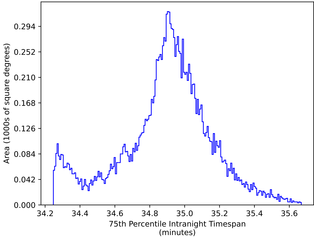
too_elab_r8_d2_ugrizy_v3.4_10yrs WFD all bands: 75th Percentile Intranight Timespan
