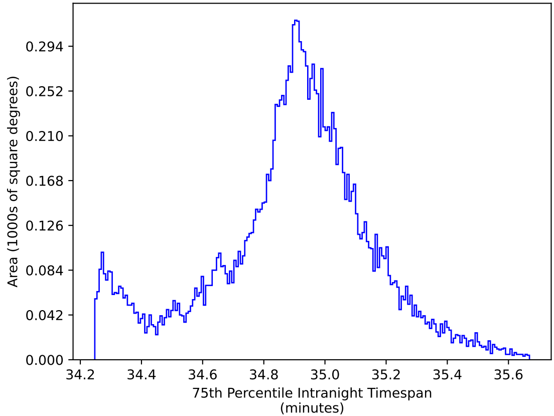
too_elab_r8_d2_ugrizy_v3.4_10yrs WFD: 75th Percentile Intranight Timespan
