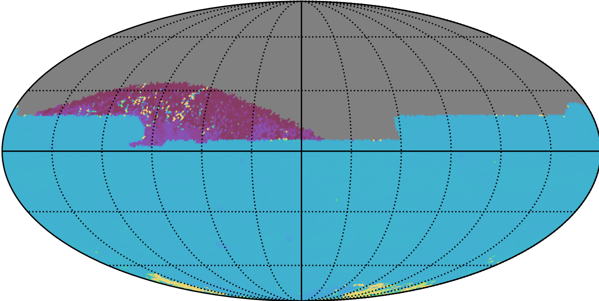
too_elab_r8_d2_ugrizy_v3.4_10yrs All sky zy bands: 75th Percentile Intranight Timespan
