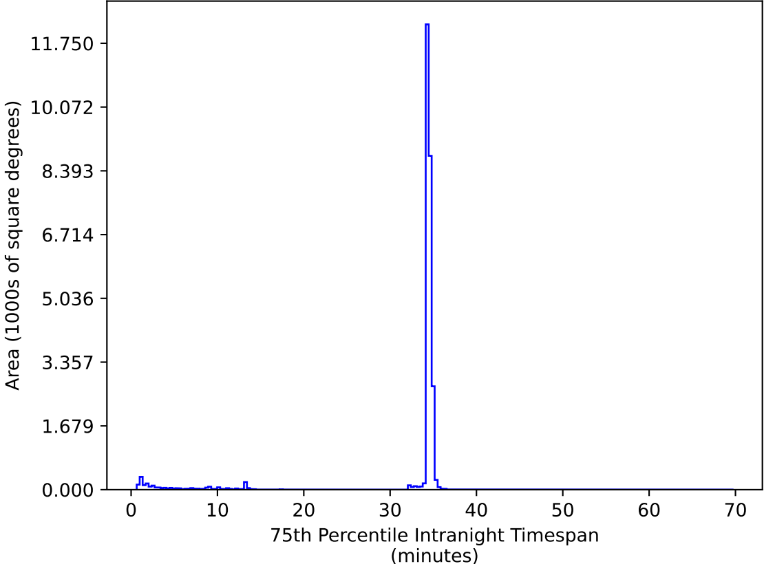
too_elab_r8_d2_ugrizy_v3.4_10yrs All sky zy bands: 75th Percentile Intranight Timespan
