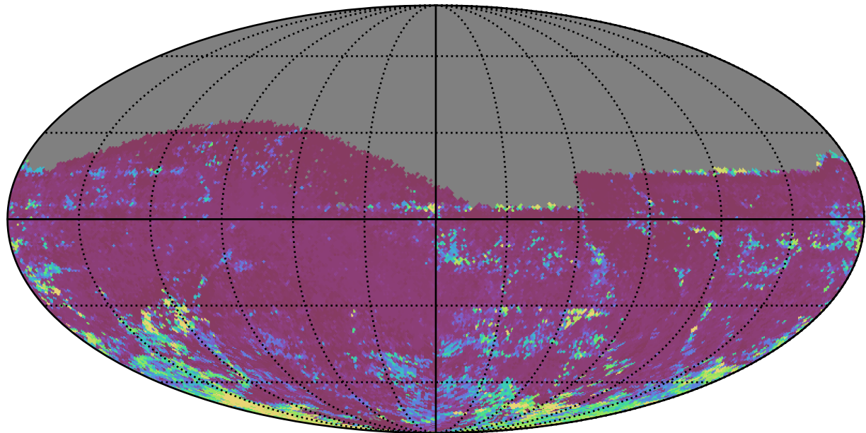
too_elab_r8_d2_ugrizy_v3.4_10yrs All sky z band: 75th Percentile Intranight Timespan
