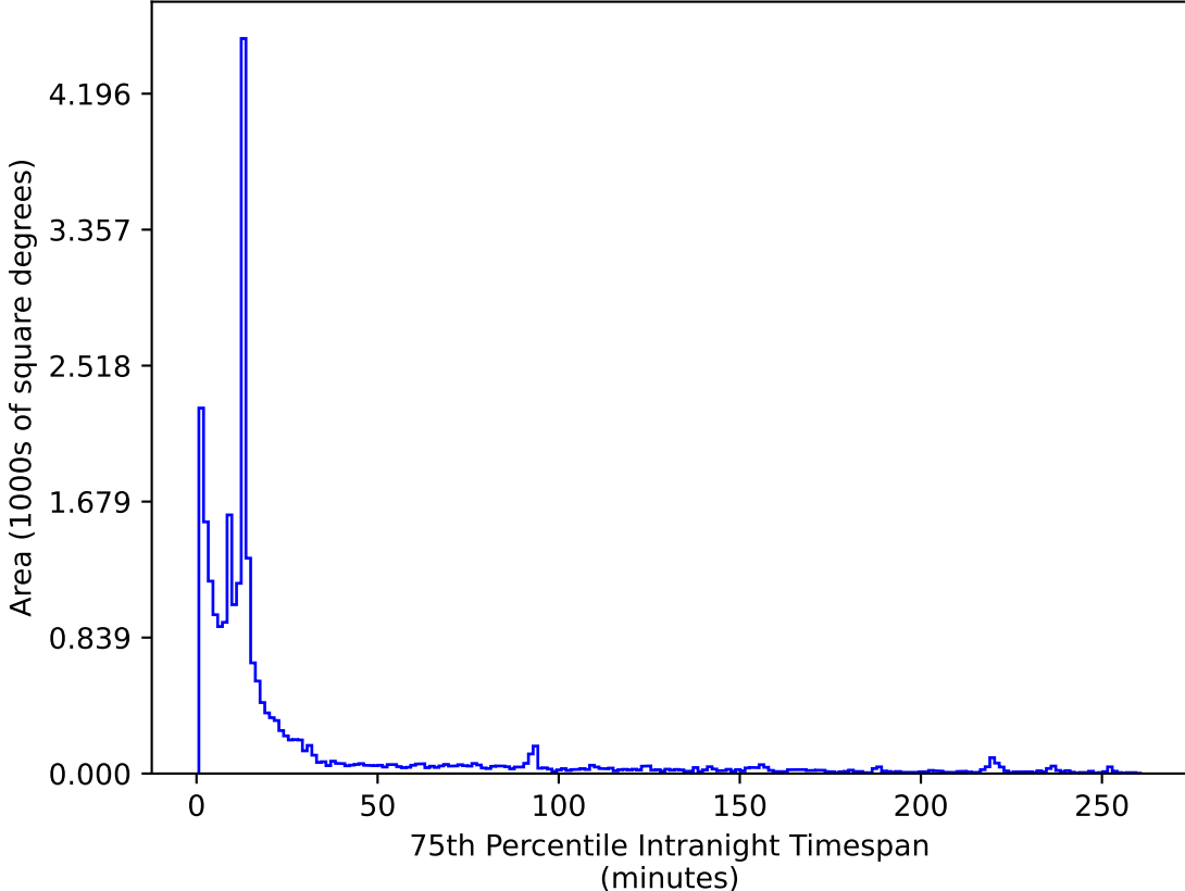
too_elab_r8_d2_ugrizy_v3.4_10yrs All sky z band: 75th Percentile Intranight Timespan
