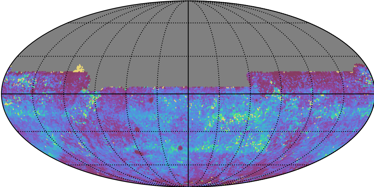
too_elab_r8_d2_ugrizy_v3.4_10yrs All sky y band: 75th Percentile Intranight Timespan
