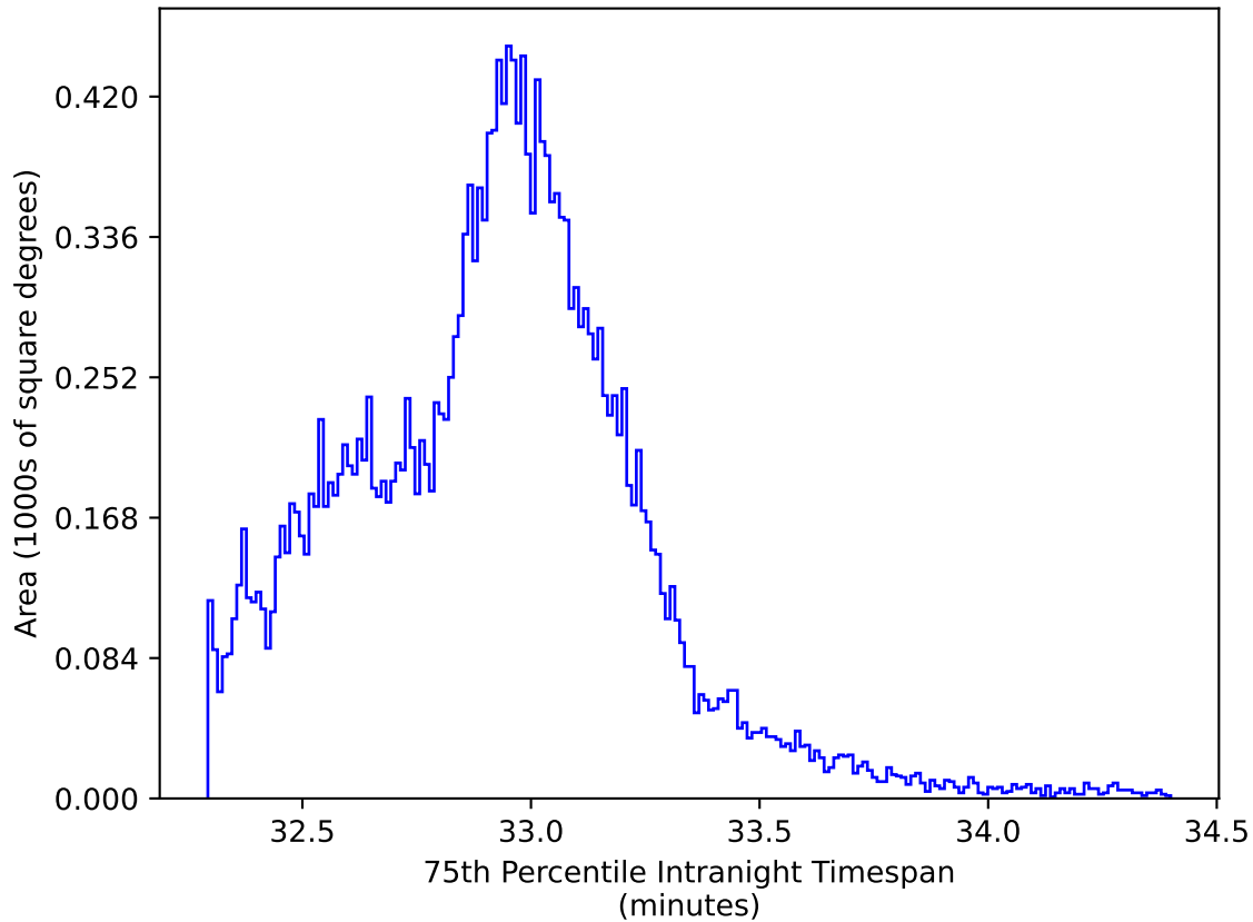
too_elab_r8_d2_ugrizy_v3.4_10yrs All sky y band: 75th Percentile Intranight Timespan
