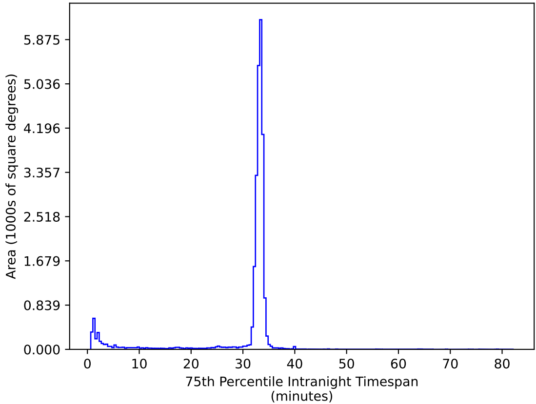
too_elab_r8_d2_ugrizy_v3.4_10yrs All sky ug bands: 75th Percentile Intranight Timespan
