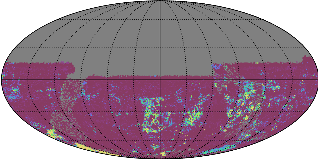
too_elab_r8_d2_ugrizy_v3.4_10yrs All sky u band: 75th Percentile Intranight Timespan
