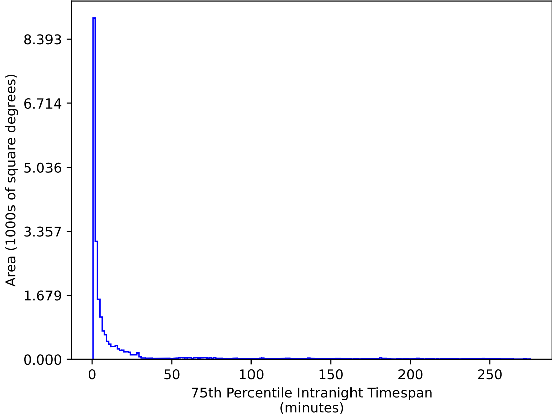
too_elab_r8_d2_ugrizy_v3.4_10yrs All sky u band: 75th Percentile Intranight Timespan
