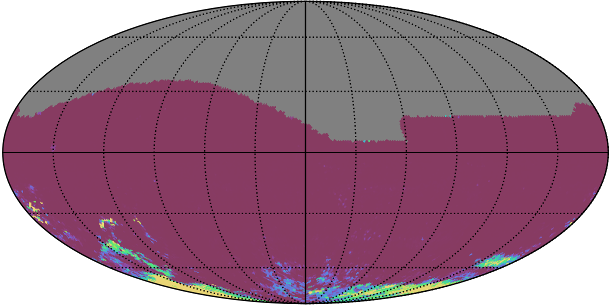
too_elab_r8_d2_ugrizy_v3.4_10yrs All sky ri bands: 75th Percentile Intranight Timespan
