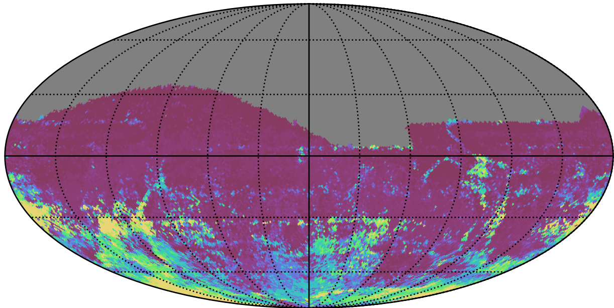
too_elab_r8_d2_ugrizy_v3.4_10yrs All sky r band: 75th Percentile Intranight Timespan
