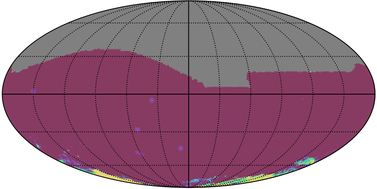
too_elab_r8_d2_ugrizy_v3.4_10yrs All sky iz bands: 75th Percentile Intranight Timespan
