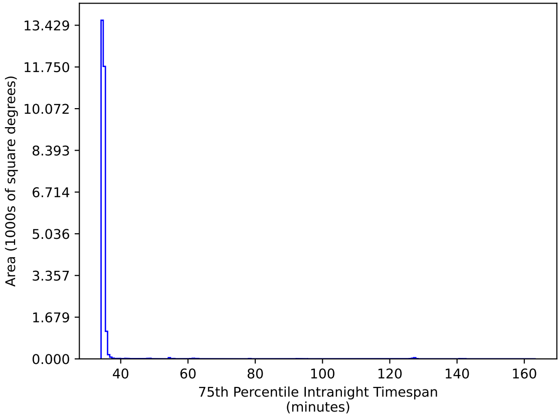
too_elab_r8_d2_ugrizy_v3.4_10yrs All sky iz bands: 75th Percentile Intranight Timespan
