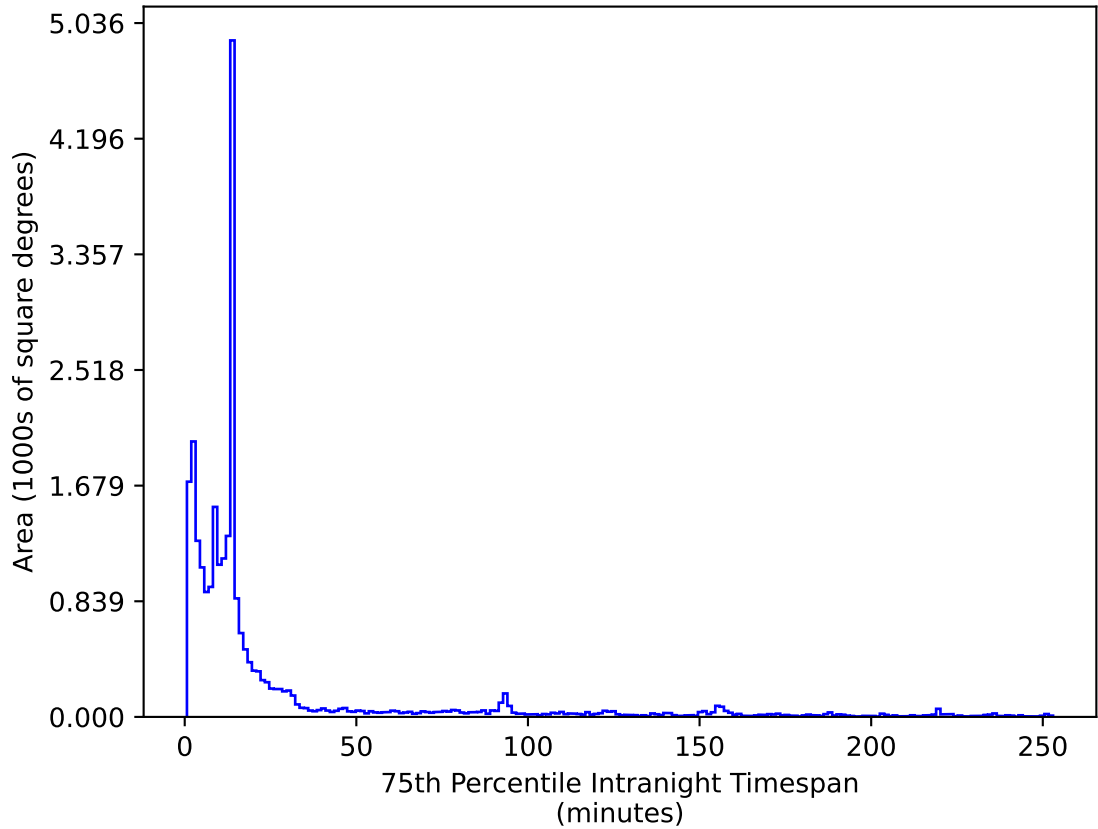
too_elab_r8_d2_ugrizy_v3.4_10yrs All sky i band: 75th Percentile Intranight Timespan
