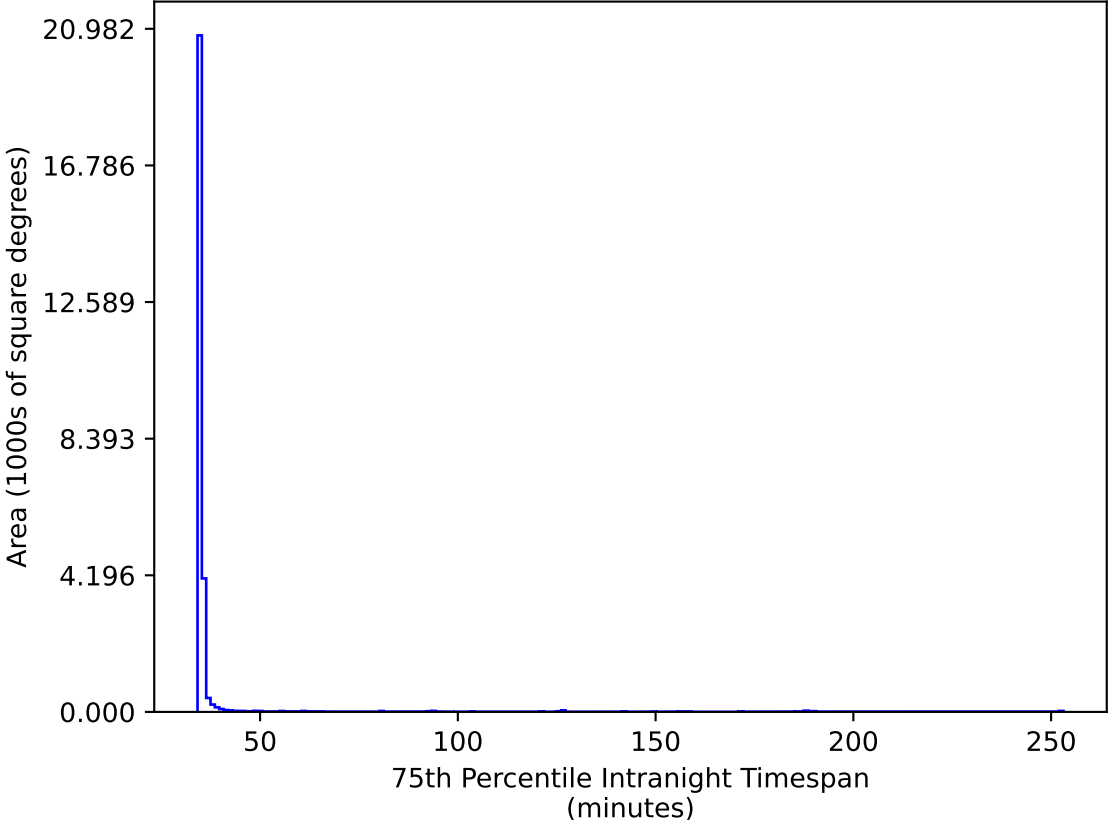
too_elab_r8_d2_ugrizy_v3.4_10yrs All sky gr bands: 75th Percentile Intranight Timespan
