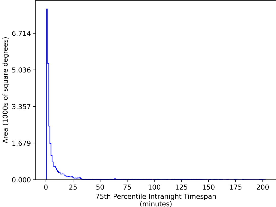
too_elab_r8_d2_ugrizy_v3.4_10yrs All sky g band: 75th Percentile Intranight Timespan
