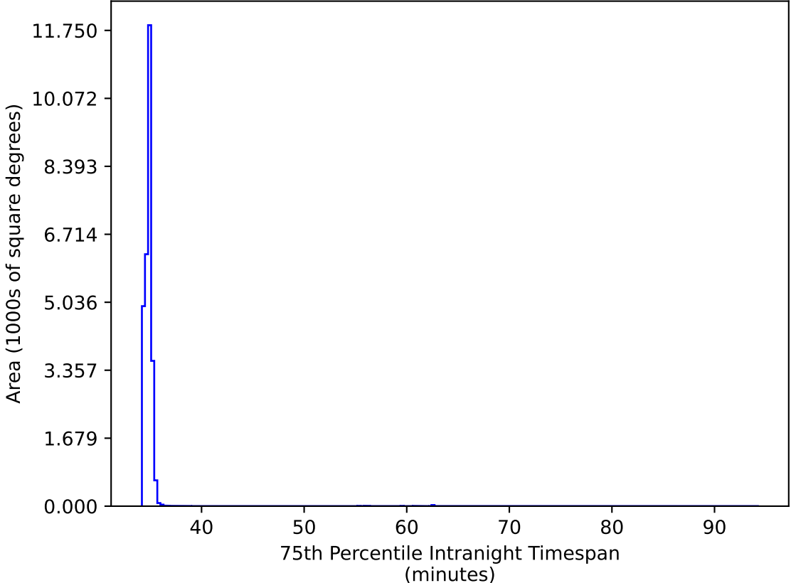
too_elab_r8_d2_ugrizy_v3.4_10yrs All sky all bands: 75th Percentile Intranight Timespan
