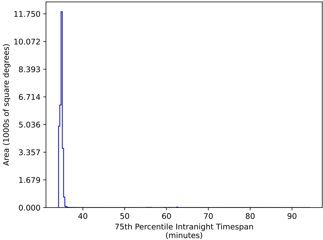
too_elab_r8_d2_ugrizy_v3.4_10yrs All sky: 75th Percentile Intranight Timespan
