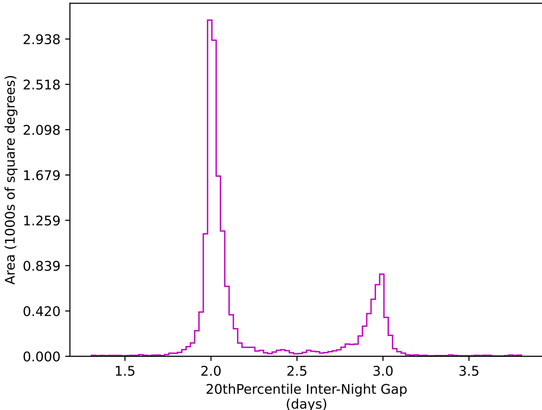
too_elab_r8_d2_ugrizy_v3.4_10yrs WFD z band: 20thPercentile Inter-Night Gap
