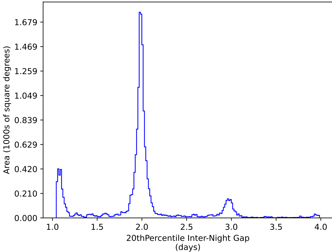
too_elab_r8_d2_ugrizy_v3.4_10yrs WFD y band: 20thPercentile Inter-Night Gap
