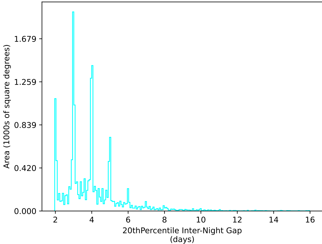
too_elab_r8_d2_ugrizy_v3.4_10yrs WFD u band: 20thPercentile Inter-Night Gap
