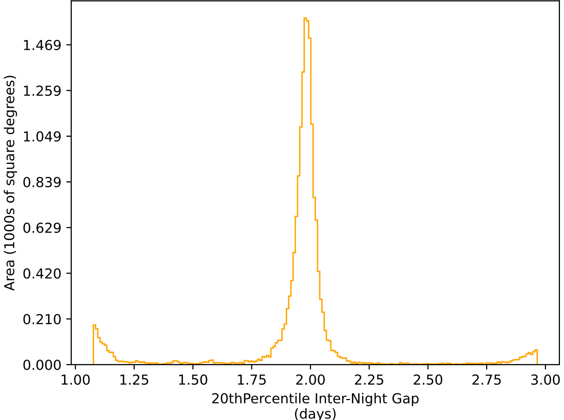
too_elab_r8_d2_ugrizy_v3.4_10yrs WFD r band: 20thPercentile Inter-Night Gap
