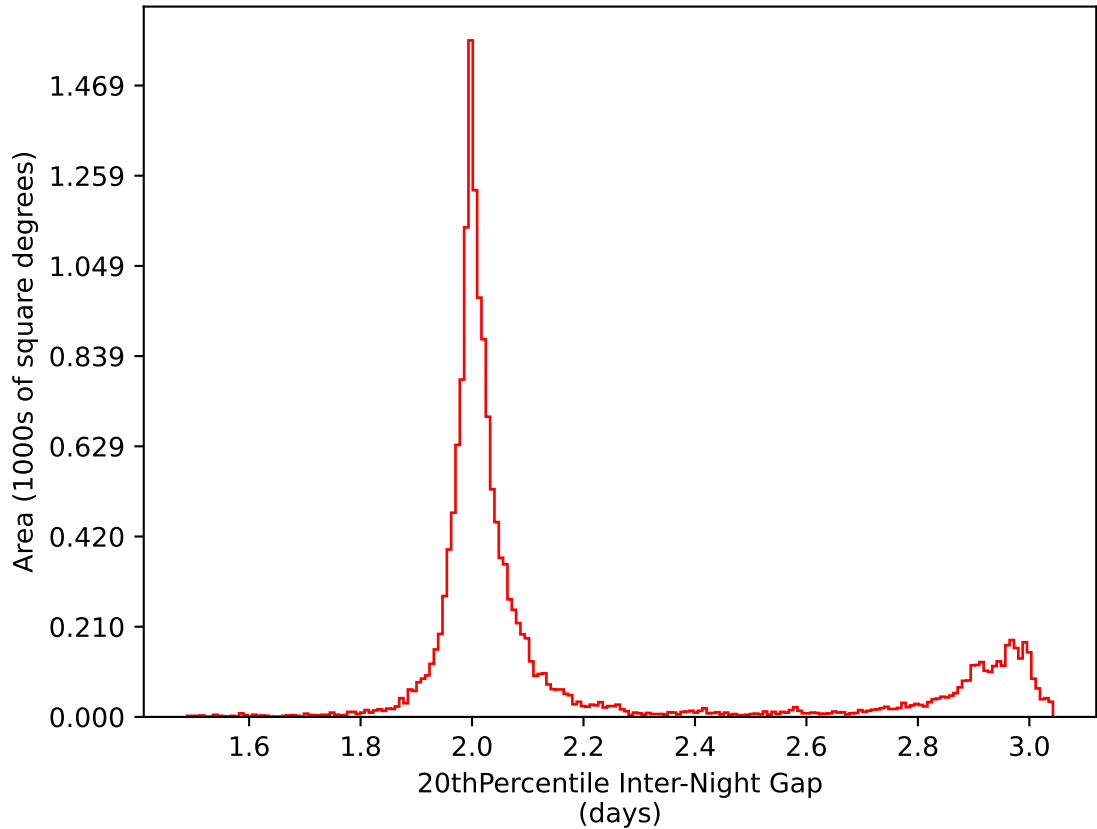
too_elab_r8_d2_ugrizy_v3.4_10yrs WFD i band: 20thPercentile Inter-Night Gap
